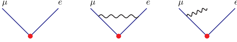
Figure 1: A sample of LO and NLO diagrams which appear for the effective \mu - e current after the neutrinos are integrated out. The factor to be associated with the effective \mu - e vertex after squaring the matrix elements is given in eq. (2.9).
